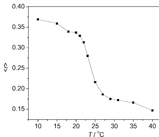
Figure 4. Fluorescence anisotropy, \langle r \rangle , of the phenyltetraene acetate 5Bb in lipid vesicles (LUV) of DMPC as a function of temperature. \lambda_{\text{exc}} = 348 nm; \lambda_{\text{em}} = 462 nm; [ 5Bb ] \approx 10^{-5} M; [DMPC] \approx 10^{-3} M; [ 5Bb ]/[DMPC] = 1:200.
