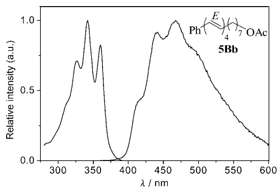
Figure 2. Absorption and corrected fluorescence spectra of all -( E )-phenyltetraene acetate 5Bb in DMSO; [ all -( E )- 5Bb ] = 2 \times 10^{-5} M (absorption), 2 \times 10^{-6} M (emission); \lambda_{\text{exc}} = 347 nm; 22 °C.
