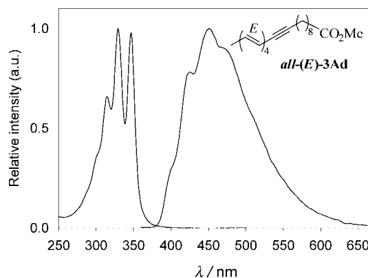
Figure 1. Absorption and corrected fluorescence spectra of the conjugated tetraenyne methyl ester all -( E )- 3Ad in CHCl 3 ; [ all -( E )- 3Ad ] = 2 \times 10^{-5} M (absorption), 2 \times 10^{-6} M (emission); \lambda_{\text{exc}} = 347 nm; 22 °C.
