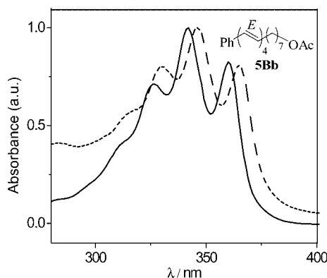
Figure 3. Absorption spectra of all -( E )-phenyltetraene acetate 5Bb in EtOH (solid line) and in large unilamellar lipid vesicles of DMPC (dashed line) at 22 °C.
